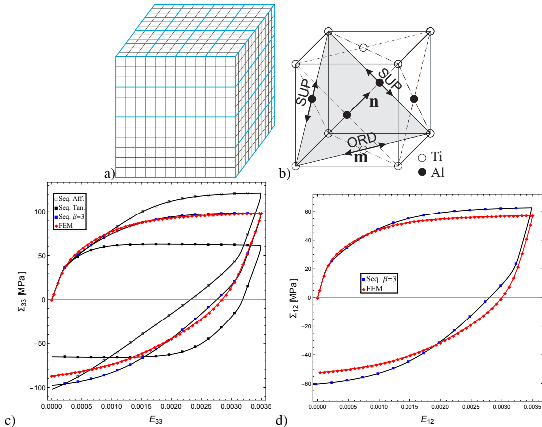
Figure 1: Example of RVE with FE mesh ( N = 64 , M = 3 ) (a); slip systems in \gamma -TiAl (ORD - ordinary dislocations, SUP - superdislocations) (b); overall response in tension-compression (c) and shear (d) cycle for \gamma -TiAl aggregate shown in (a) with exponent n = 8 in the local power law and an anisotropy factor \alpha = 5 .
