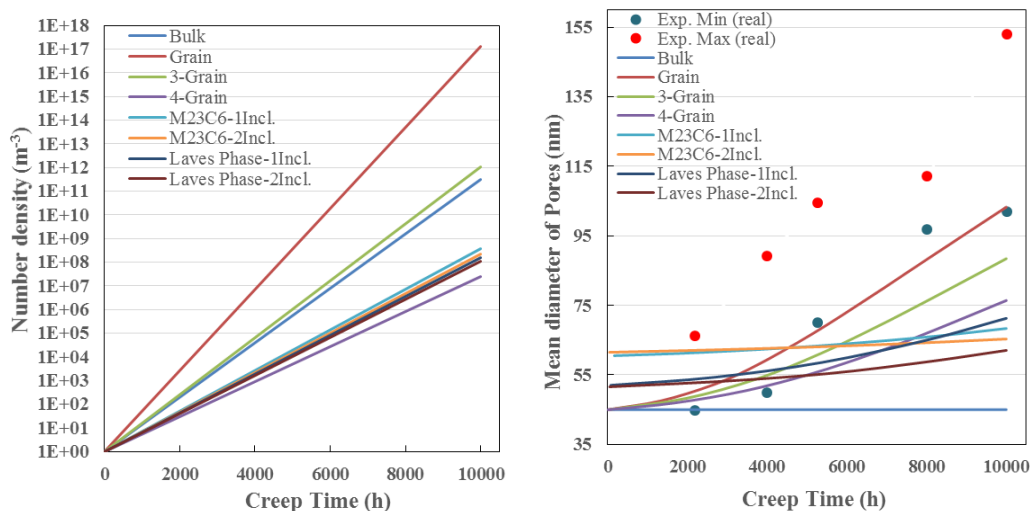
Fig. 3. Simulated results of (a) number density and (b) size of the formed pore in different regions of the crept material such as bulk, grain, 3-grain, 4-grain, \text{M}_{23}\text{C}_6 and Laves phase after 10,000 hours creep at 650°C and under 66 MPa tension.
