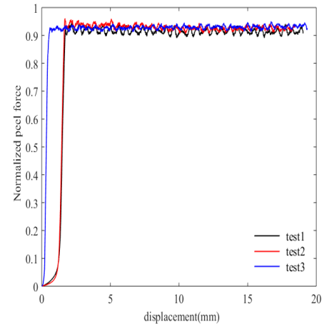
Fig.3: Evolution of the normalized peel force measured during a 90° peel test. After a few millimeters of crosshead displacement, a steady state is established.
