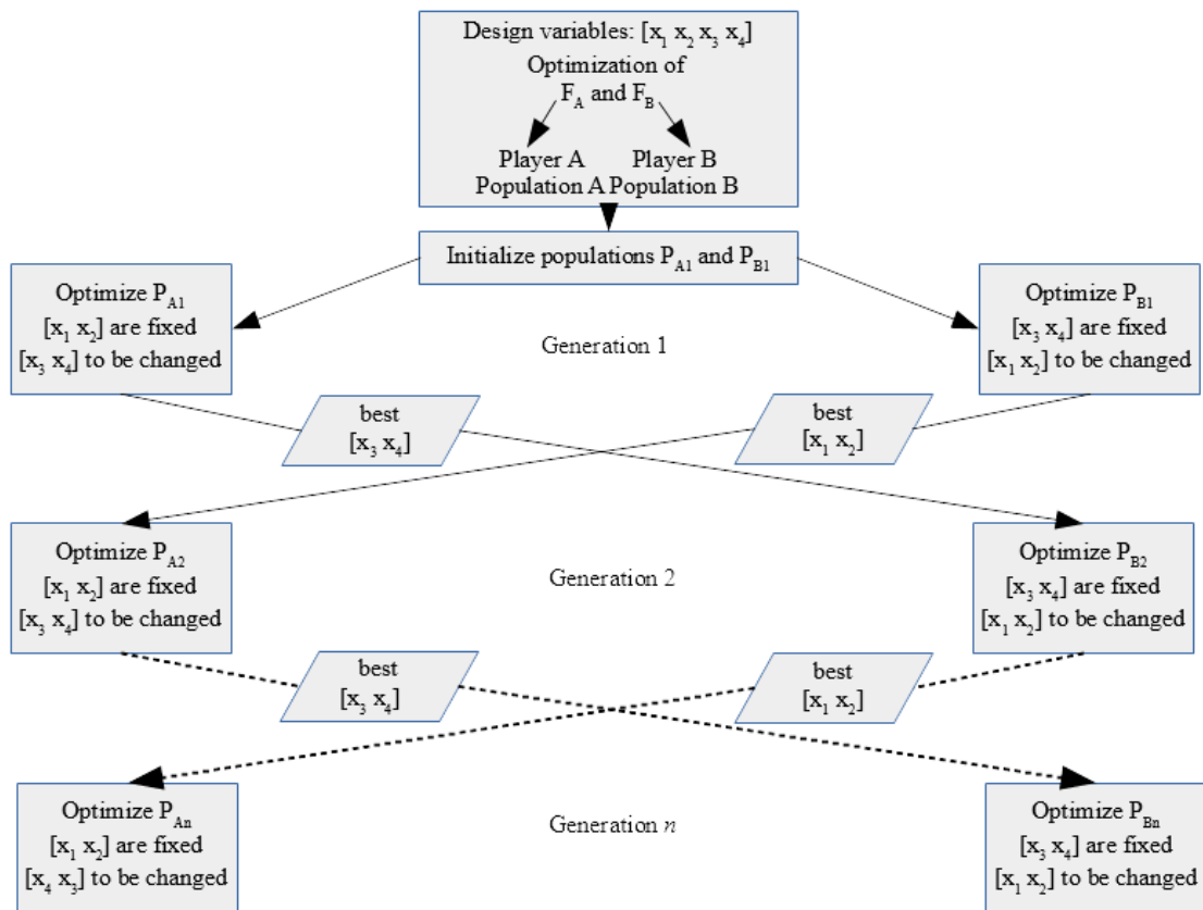
Figure 1: Coupled differential evolution and game theory multiobjective optimization algorithm.
